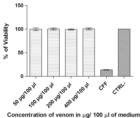
Figure 3 MTS metabolism in HeLa cells after treatment with different doses of venom (50-400 µg/100 µL of medium), positive control (CFF, cyclophosphamide 400 µg/100 µL) and negative control (CTRL-). Optical density (OD) was read at 490 nm, the data were plotted according to the mean and SD. Treatment means differed significantly with respect to the positive control but not for the negative control ( p < 0.05 ).
