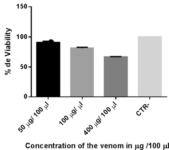
Figure 4 MTS metabolism by macrophages and viability percentage showed significant difference between treatment means at p < 0.05 .
